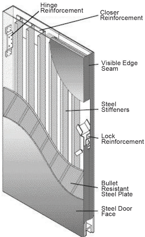
Steel Bullet Resistant Door
