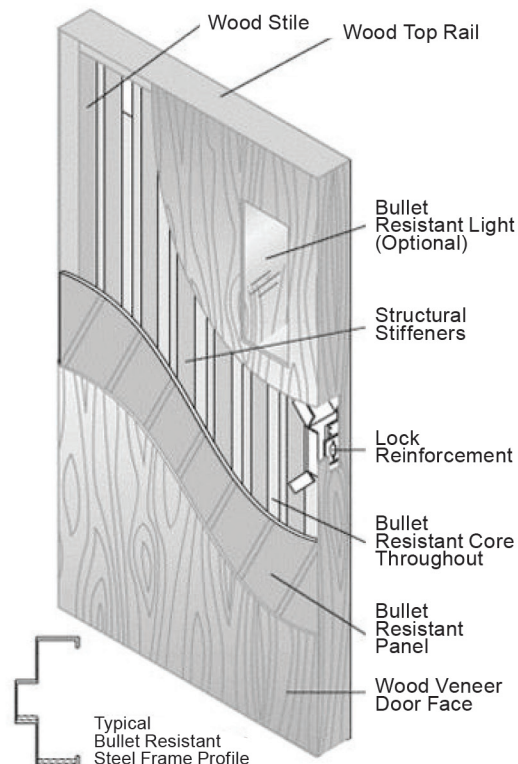
Wood Bullet Resistant Door
